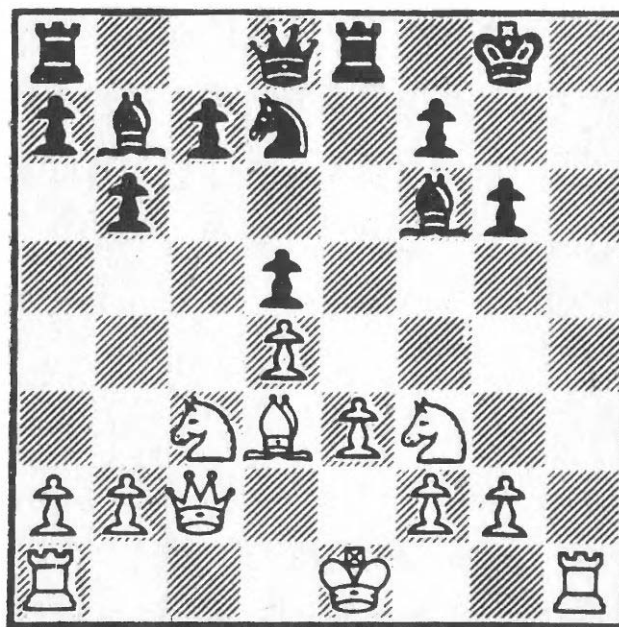
455 After 13...Nd7
